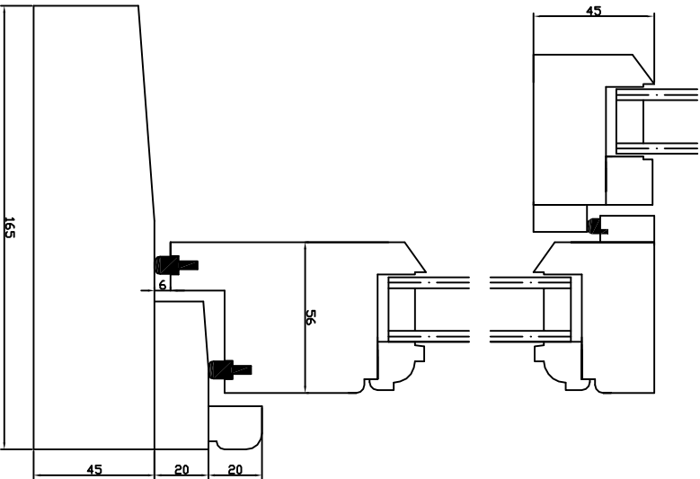
Sash - vertical section
